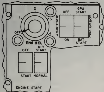
FIGURE 5-16. Engine start panel.
